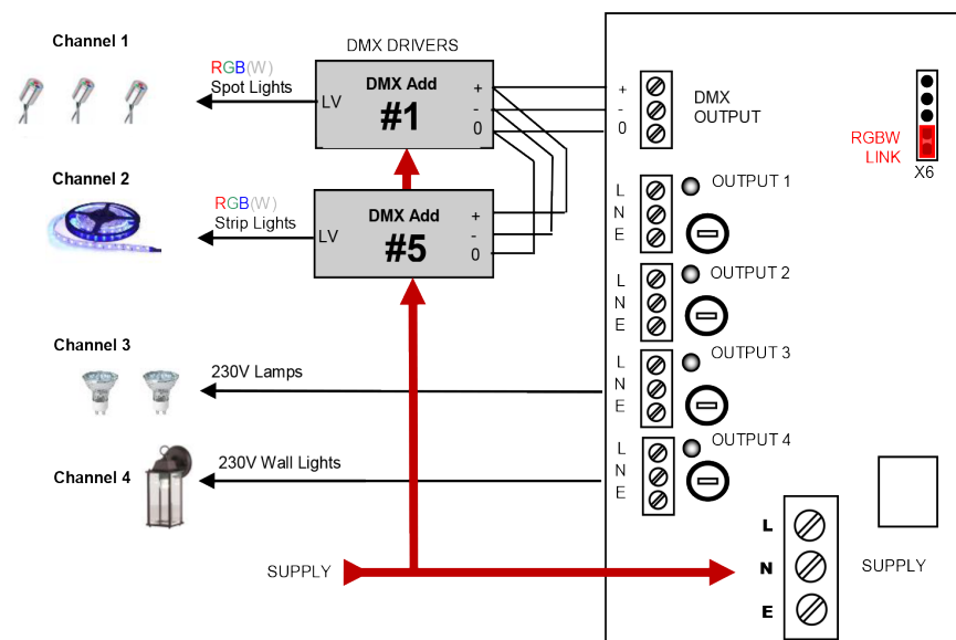
EXAMPLE WIRING
